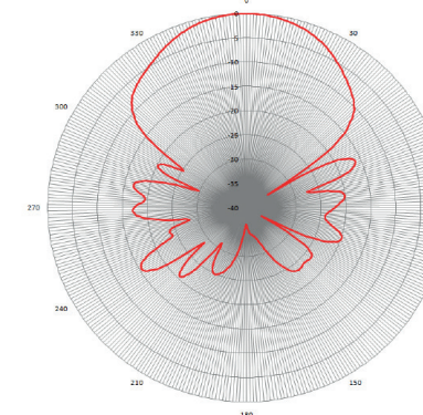
Horizontal 1850MHz 0dB = 12 dBi
